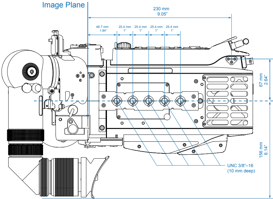
Camera Top
