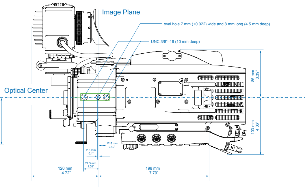
Camera Bottom
