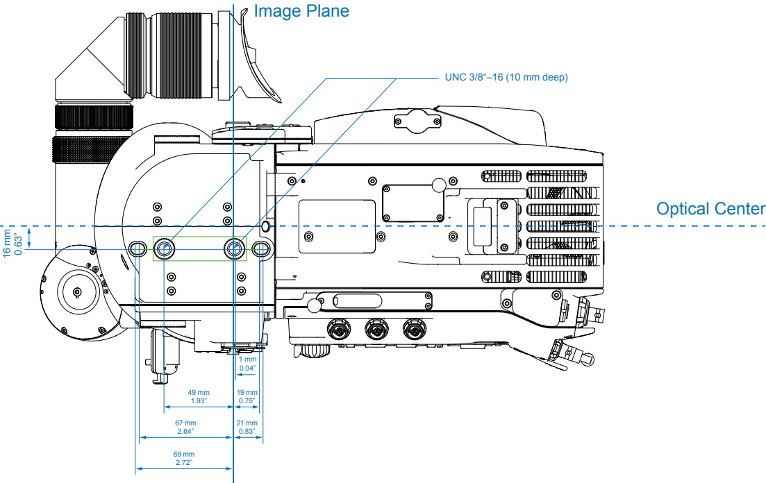
Camera Bottom
