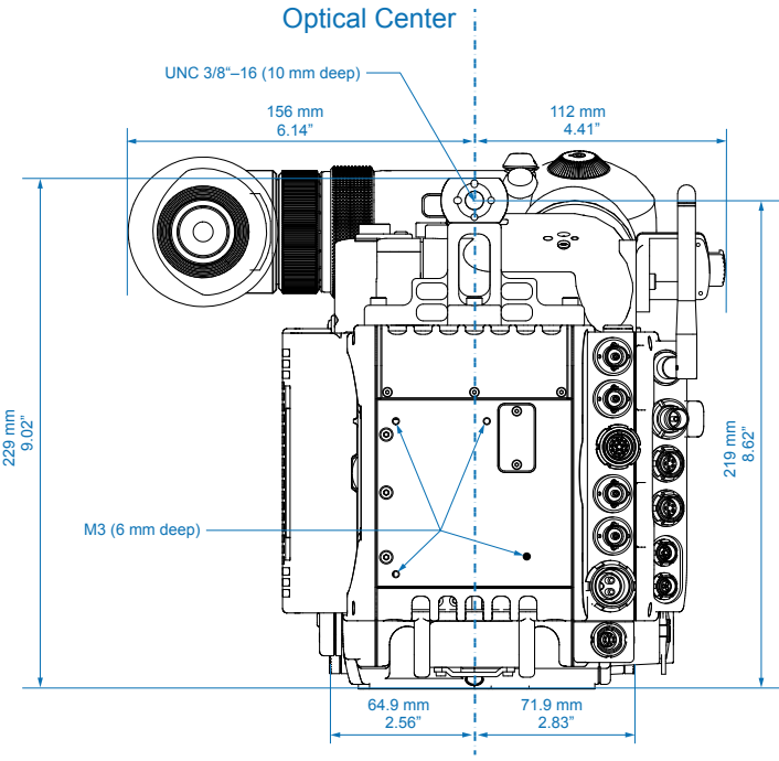
Camera Back
