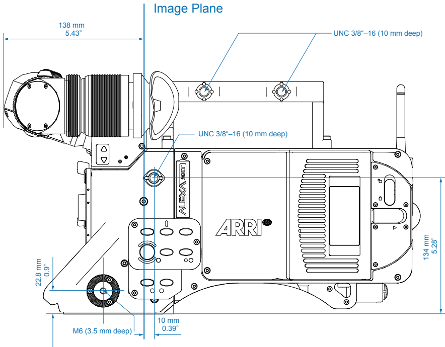
Camera Left
