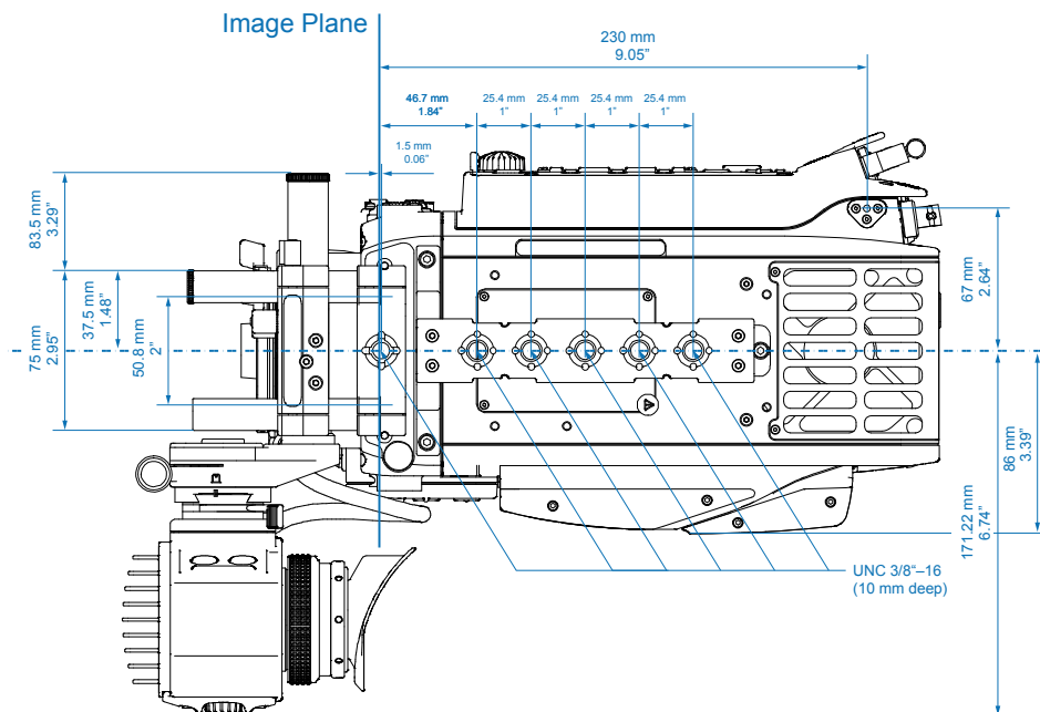
Camera Top
