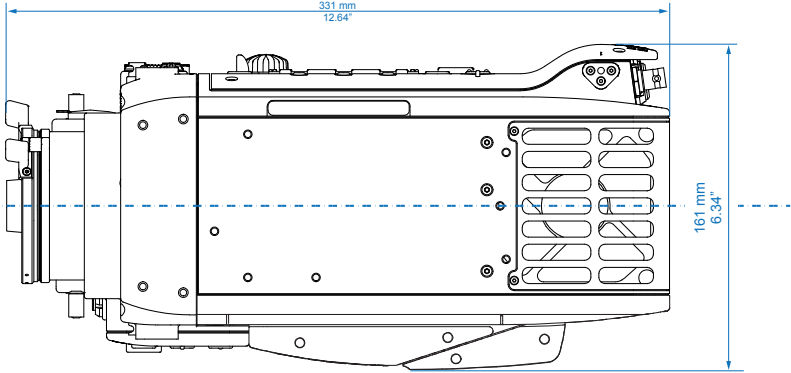
Optical Center
