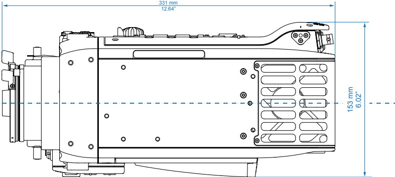
Optical Center
